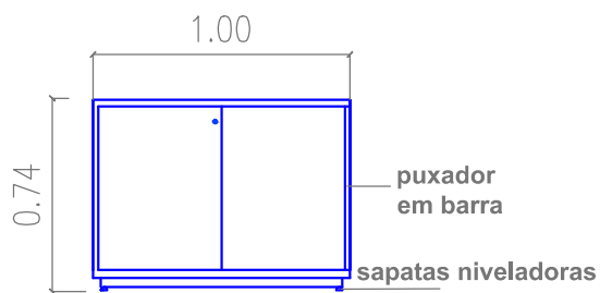
Vista frontal
