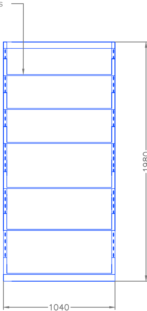
VISTA FRONTAL
